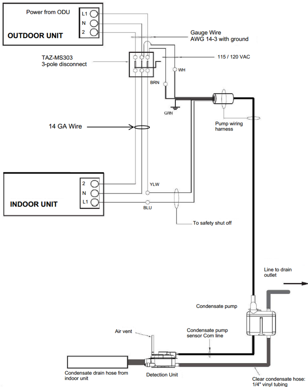
Figure 1. X87-711 or Si-30-120V Wiring Diagram
