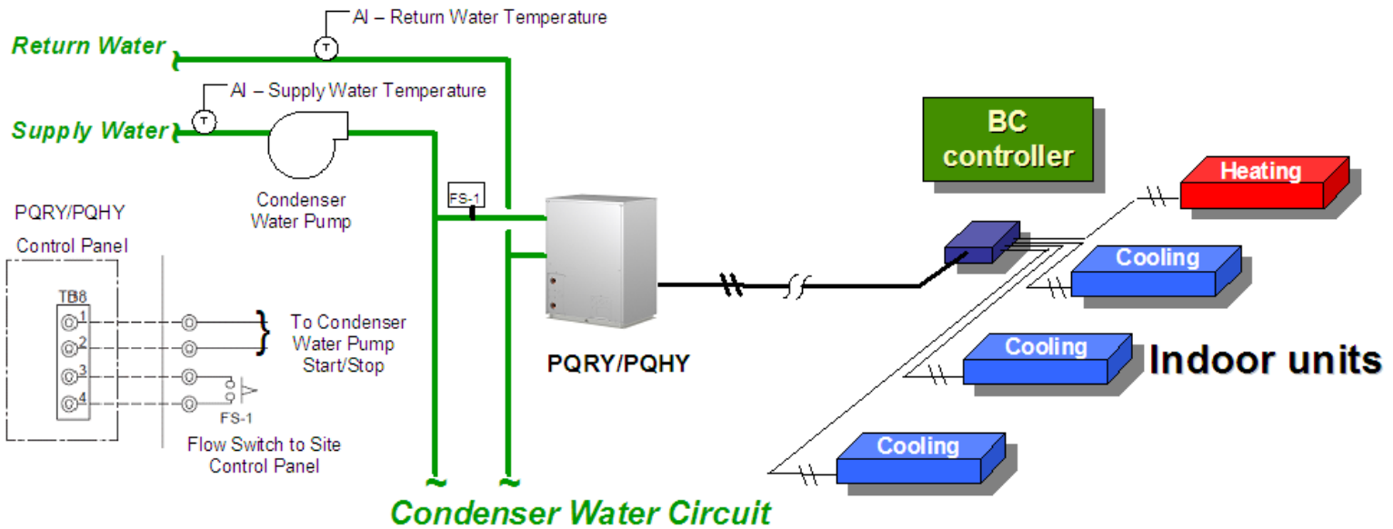
Figure 1. Input/Output (I/O) Controller and W-series (PQR/PQHY) Outdoor Units
