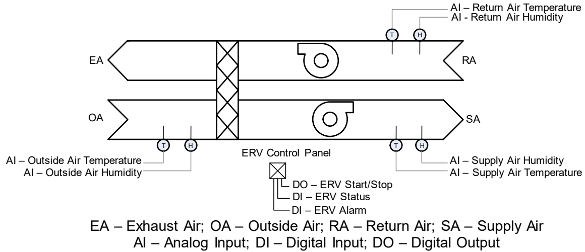
Figure 1. Energy Recovery Ventilators (ERV) Control
