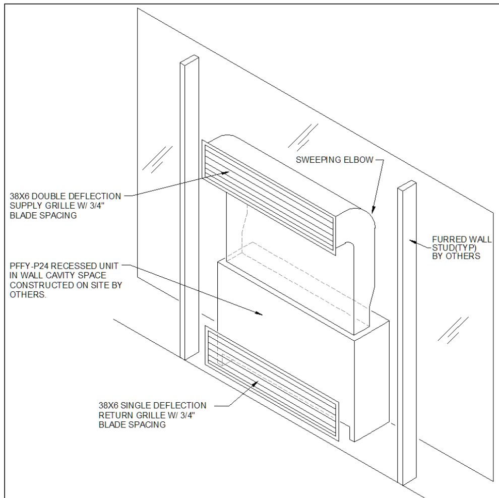
Figure 1 – Example PFFY-P24 (500 CFM) Concealed Installation
