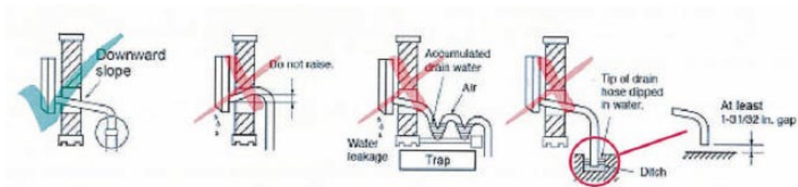
Figure 1. Condensate drain pipe connection
