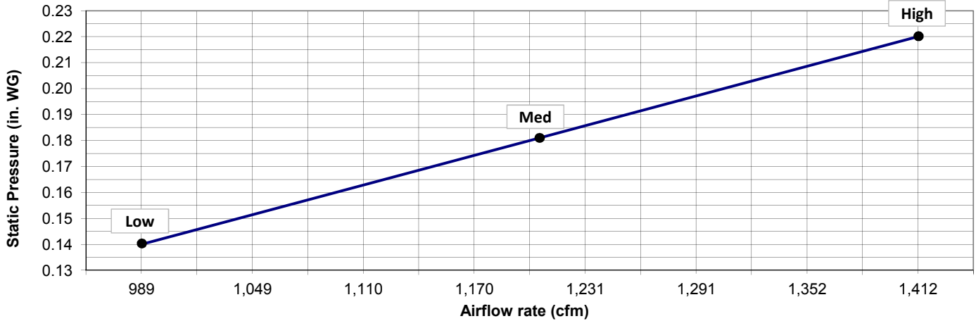
PEFY-P48-NMAU-E3 with Filter Box FBM2-4
