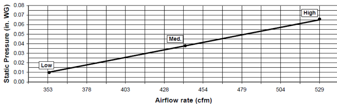
SEZ-KD15NA with Filter Box FBL1-2
