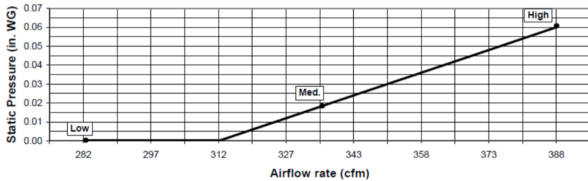
SEZ-KD12NA with Filter Box FBL1-2
