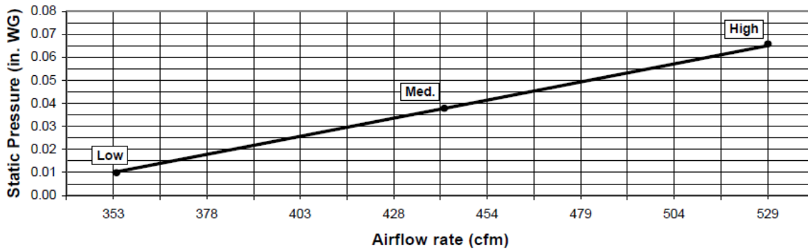
PEFY-P18NMSU-ER2 with Filter Box FBL1-2
