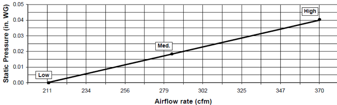
PEFY-P12NMSU-E with Filter Box FBL1-1
