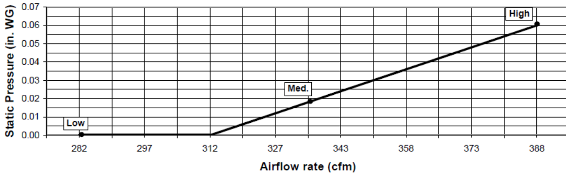
PEFY-P15NMSU-ER2 with Filter Box FBL1-2
